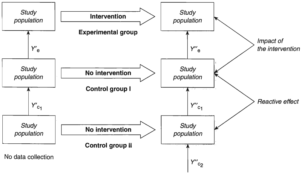
FIGURE 8.11 Double-control designs
