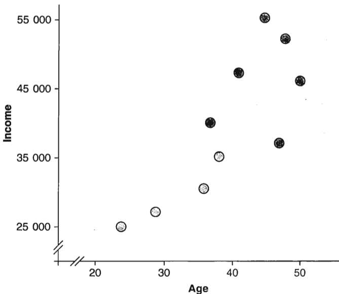
FIGURE 16.12 The scattergram
