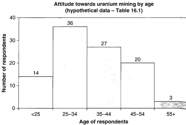
FIGURE 16.2a Two-dimensional histogram
