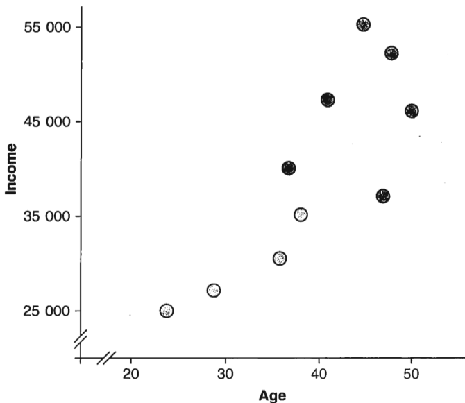
FIGURE 16.12 The scattergram
